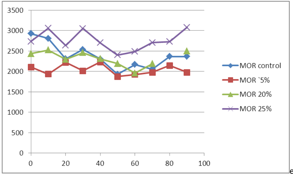
Figure 2 – Modulus of Rupture Stress vs. Time Aged at 50°C
