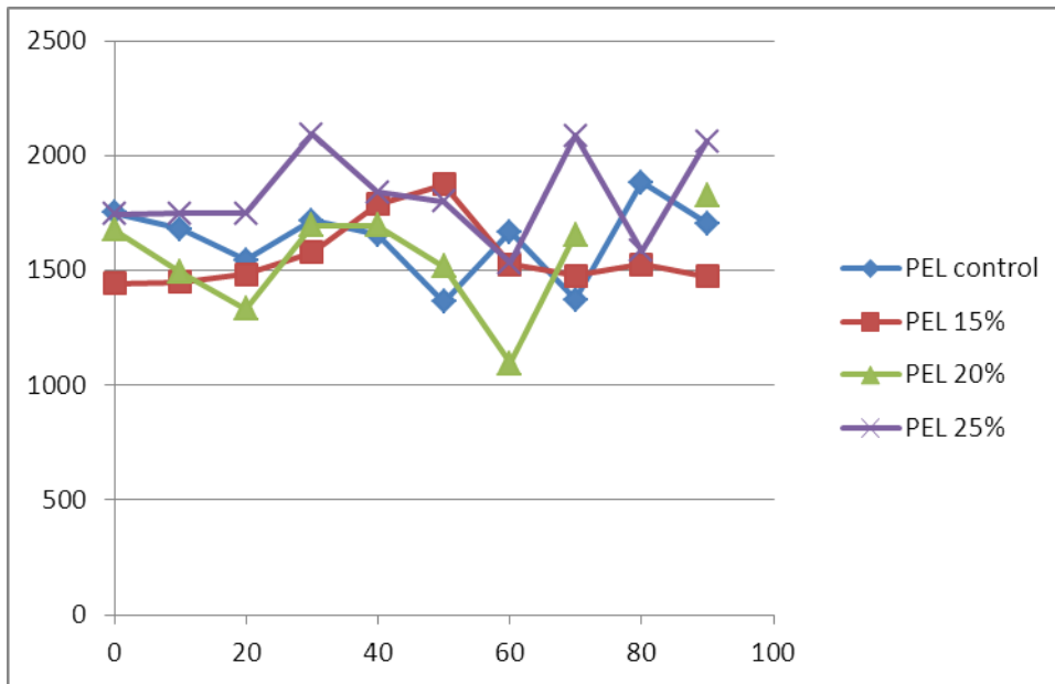
Figure 3 – Proportional Elastic Limit Stress vs. Time Aged at 50°C
