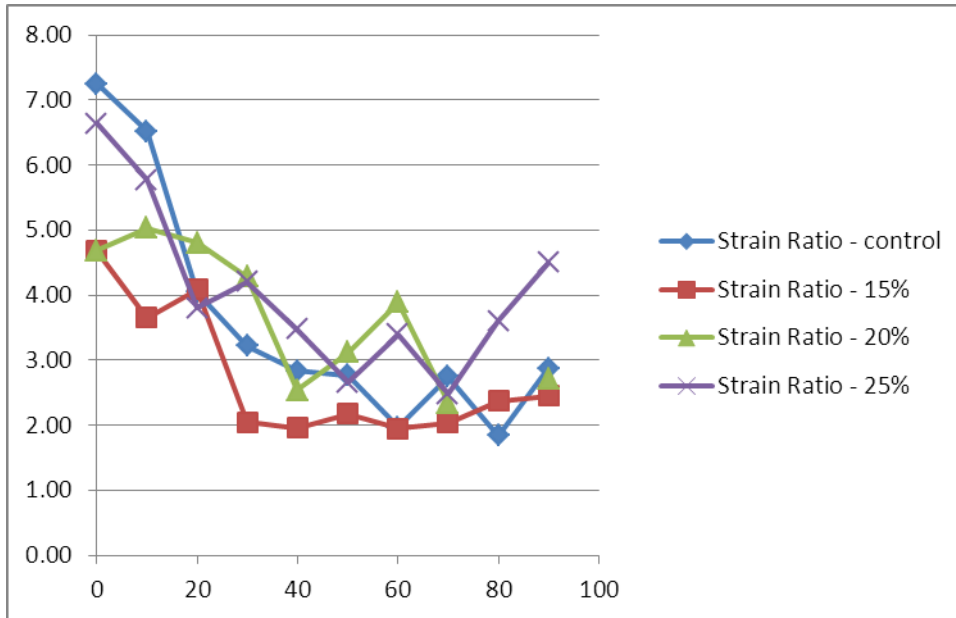
Figure 5 – Ratio of Modulus of Rupture Strain to Proportional Elastic Limit Strain vs. Time Aged at 50°C
